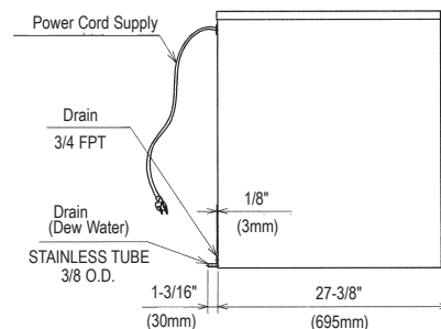
KM-280 SIDE VIEW
