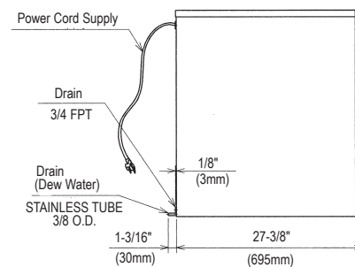
KM-500 SIDE VIEW
